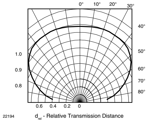
Fig. 12 - Vertical Directivity
