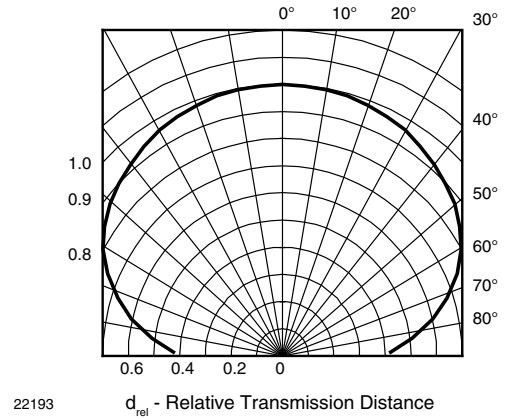
Fig. 11 - Horizontal Directivity
